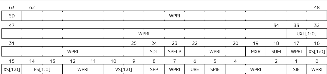
Figure 67. Virtual supervisor status ( vsstatus ) register when VSXLEN=64 .
