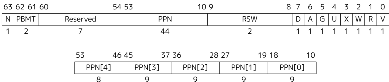
Figure 44. Sv57 page table entry.
