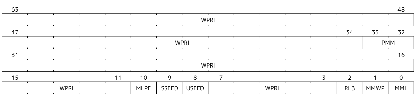
Figure 2. Machine security configuration ( mseccfg ) register.
