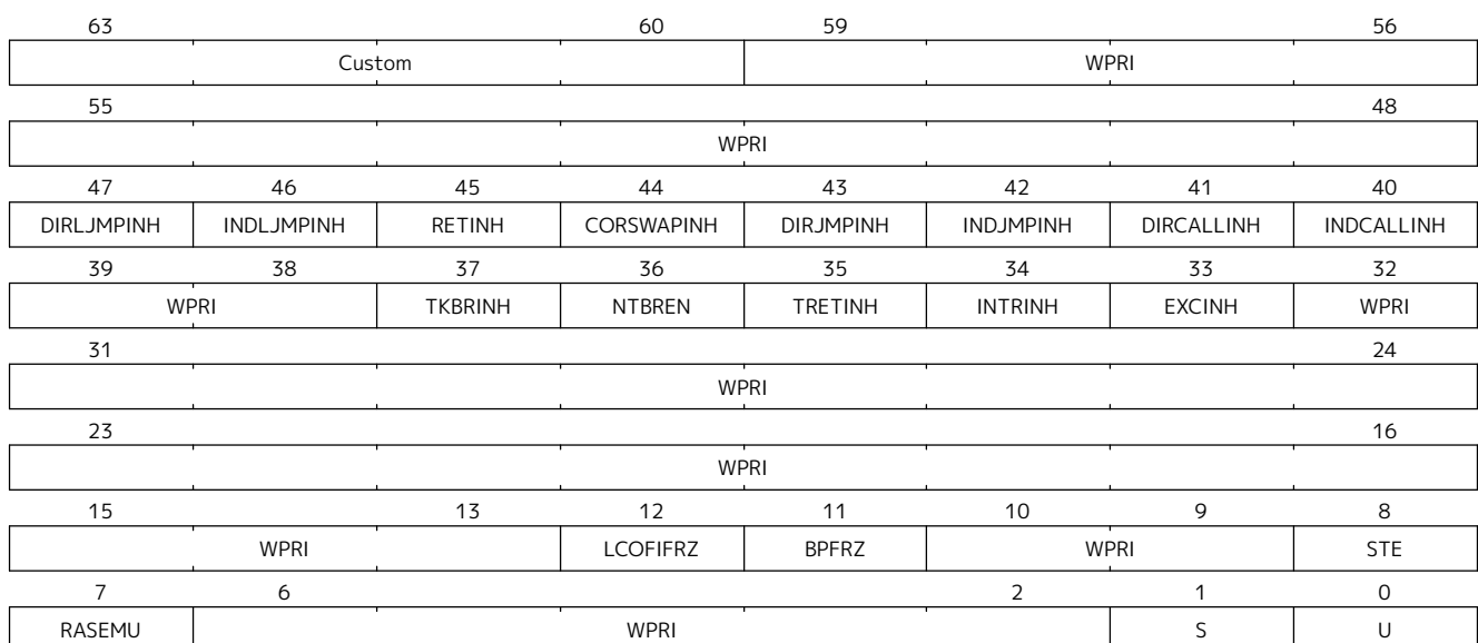
Figure 11. Virtual Supervisor Control Transfer Records Control Register Format
